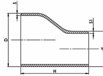
Eccentric Reducer
