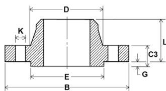
WELDING NECK
