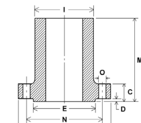
LONG WELD NECK
