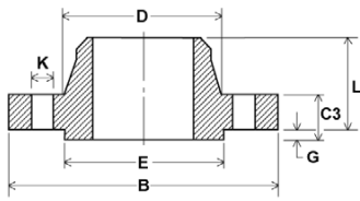
WELDING NECK
