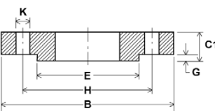
PLATE SLIP-ON WELDING
