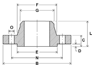
WELDING NECK
