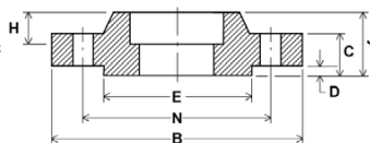
SOCKET WELDING
