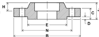
SOCKET WELDING
