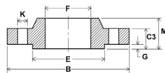
BOSSED
