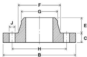
WELDING NECK
