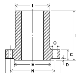
LONG WELD NECK
