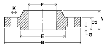
BOSSED
