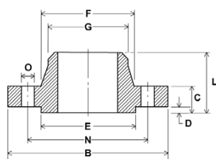
WELDING NECK
