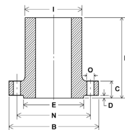
LONG WELD NECK
