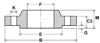
BOSSED
