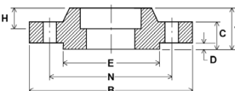
SOCKET WELDING
